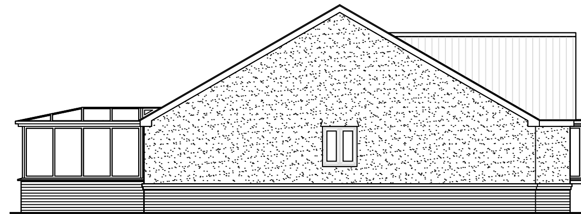
SIDE ELEVATION
